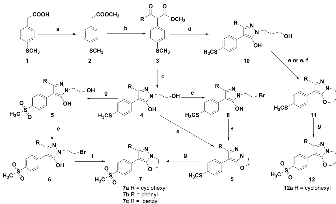
Scheme 1. (a) MeOH, c. H 2 SO 4 , rfx, 16 h; (b) LiHMDS, RCOCl, THF; (c) gl. acetic acid, NH 2 NH(CH 2 ) 2 OH, 100 °C, 1 h; (d) gl. acetic acid, NH 2 NH(CH 2 ) 3 OH, 100 °C, 1 h; (e) polymer supported-PPh 3 , CBr 4 , DMF, rt, 3 days or CBr 4 , PPh 3 , CH 2 Cl 2 , rt, 3 days; (f) K 2 CO 3 /DMF, rt, 1 h; (g) Oxone, MeOH/H 2 O, rt.
